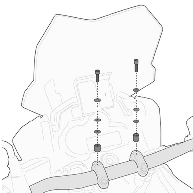
02SKITK Specific kit to mounting the KS900A Smart Bar
