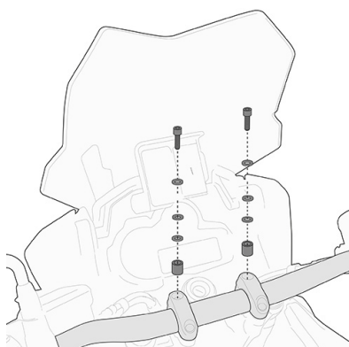
01SKITK Specific kit to mounting the KS900A Smart Bar
